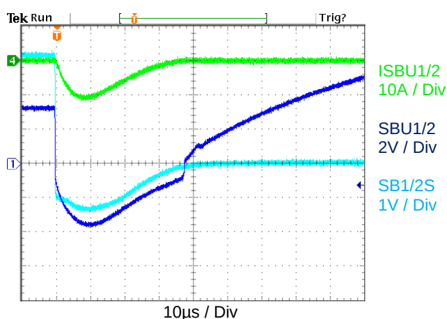
SBU -30V Surge Event
