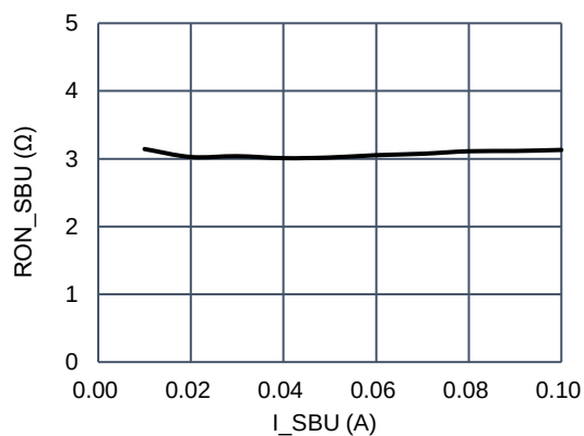
SBU Switch R_{ON} vs. Switch Current
