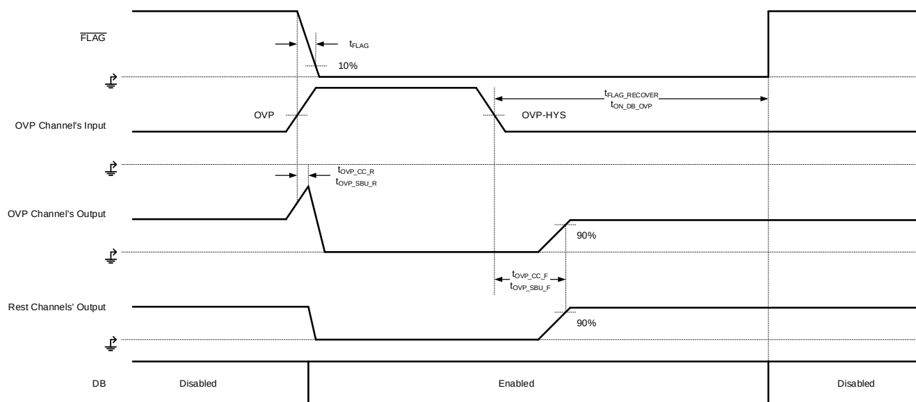
Figure 2. OVP
