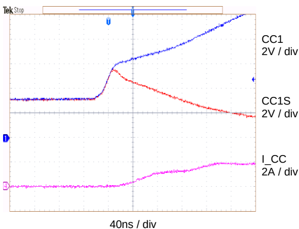
Hot-plug CC1 to 20V
