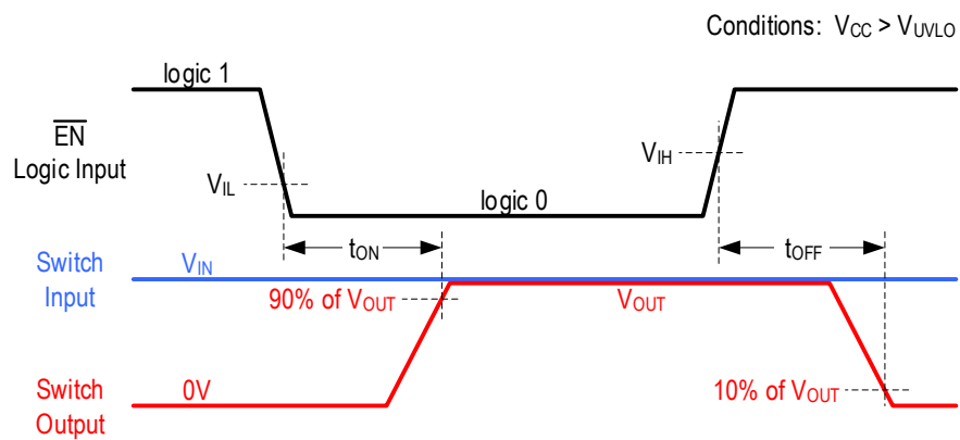
Figure 2. Switch Enable/Disable (via \overline{EN} falling/rising) Timing Diagram
