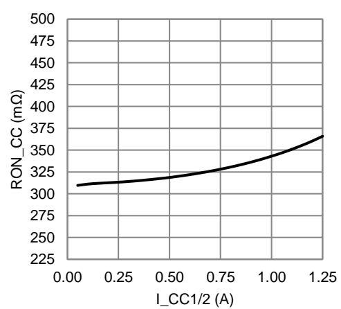
CC Switch Ron vs. Switch Current
