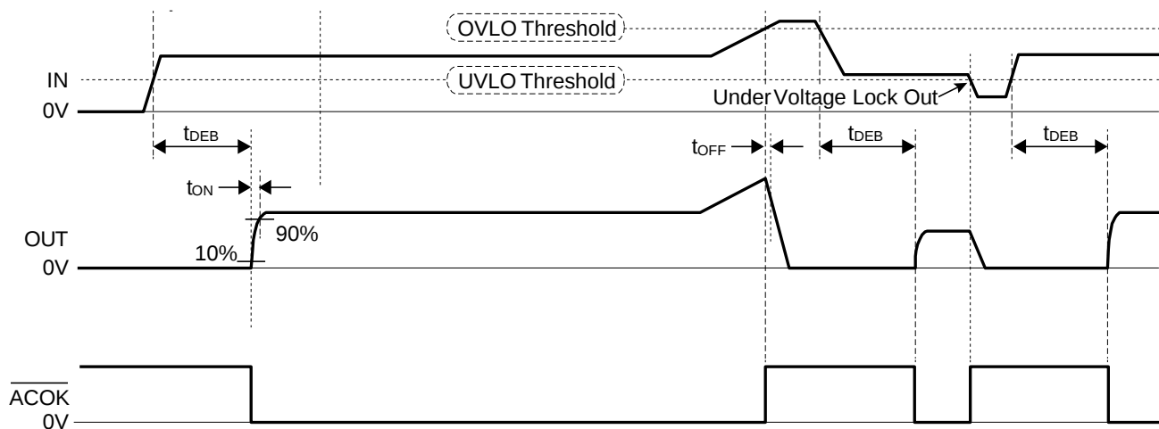
Figure 1. Timing Diagram
