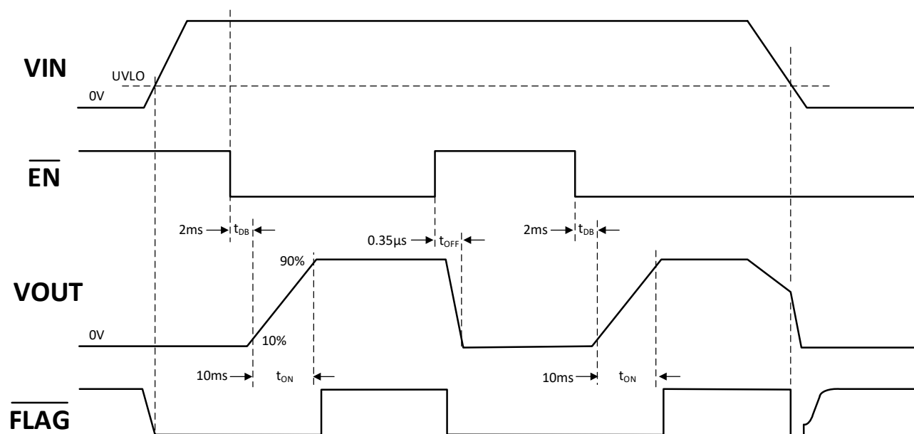
Figure 1. TURN-ON/TURN-OFF, When initially VIN = 0V, EN = H
