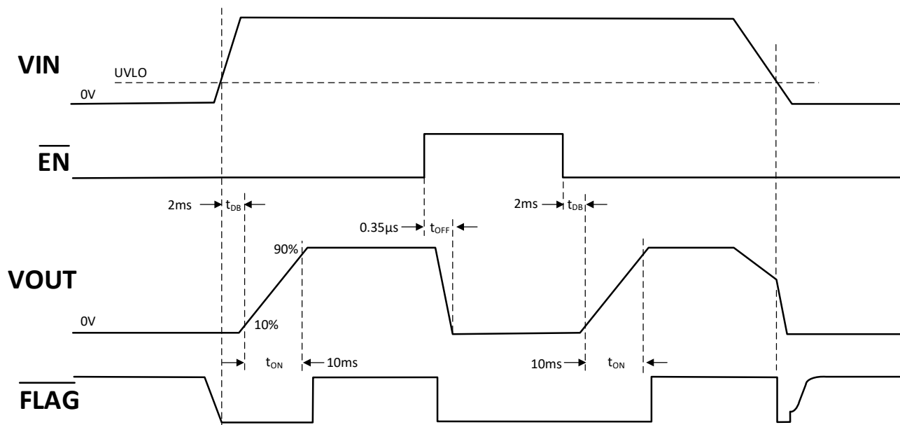
Figure 2. TURN-ON/TURN-OFF, When initially V_{IN} = 0V , \overline{EN} = L
