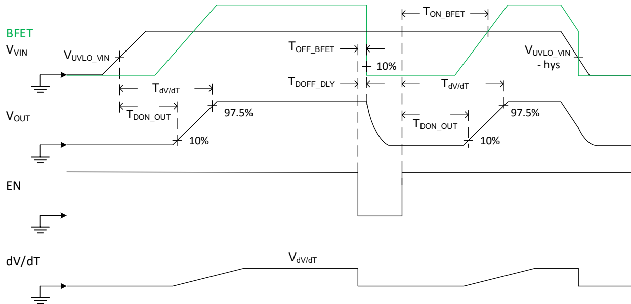
Figure 1. VIN Ramp-up, Ramp down and EN Toggling
