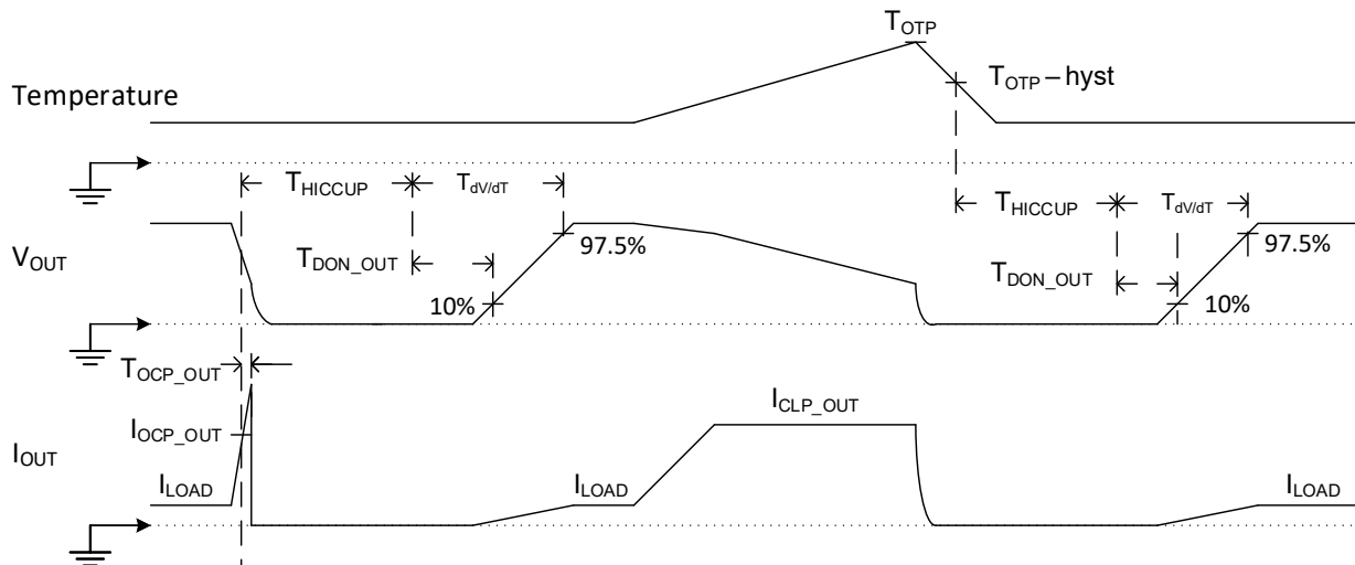
Figure 2. OCP, CLP and OTP Timing Diagram
