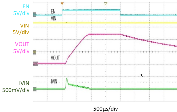
CLP Response (2.1A Current Limit, R_{SET} = 45.3k\Omega )
