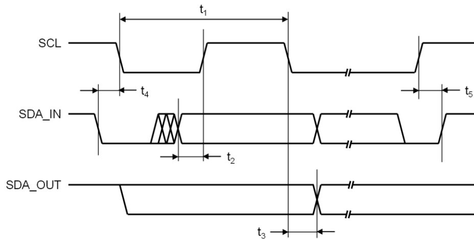
Figure 1. I²C Compatible Interface Timing Diagram
