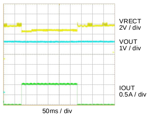
BPP, V_{OUT} = 5V , 0 to 1A Load Transient
