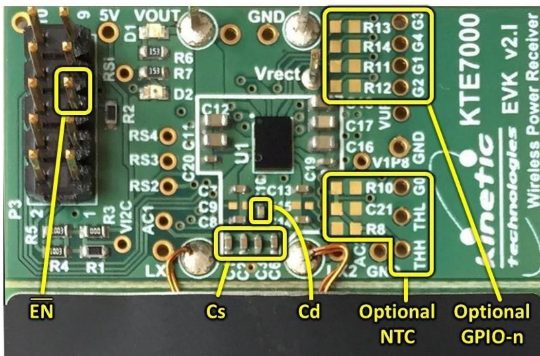
Figure 4. Photo of Evaluation Kit
