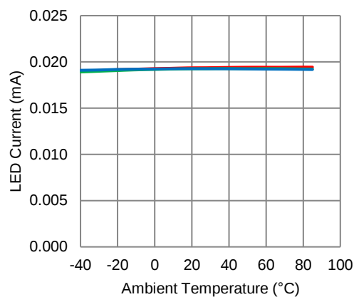
LED Current (20mA) vs. Temperature
