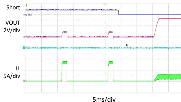
Output Short Recovery Output Short to 2A Load, V_{OUT} = 3.3V
