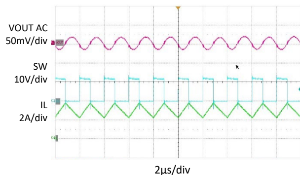
Switching waveform 3A load
