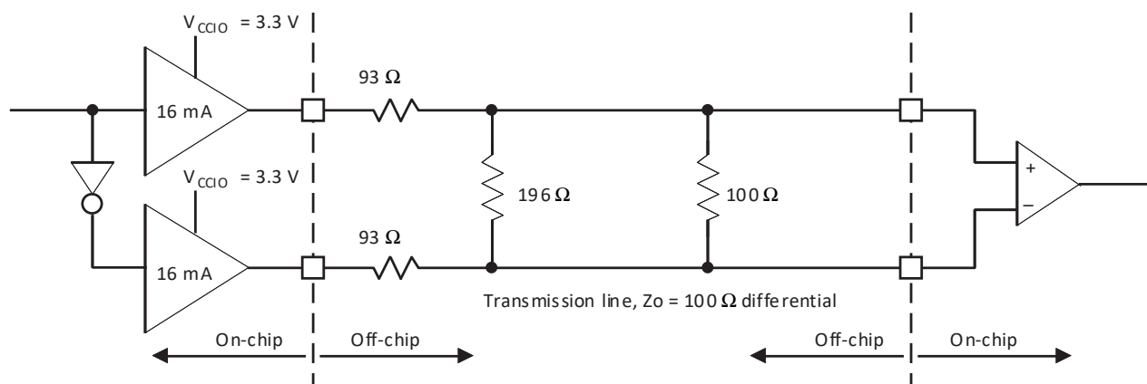
Figure 3.3. Differential LVPECL
