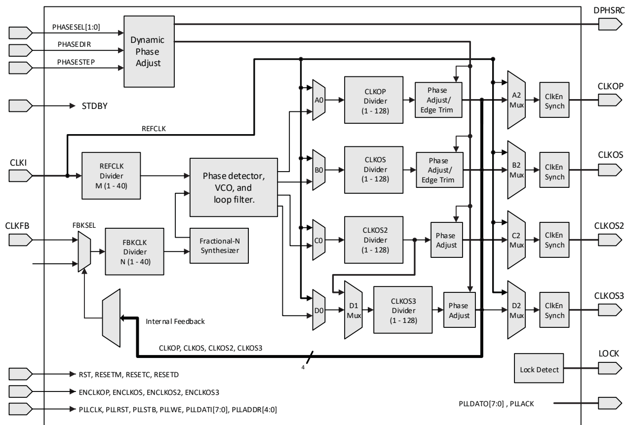
Figure 2.6. PLL Diagram
