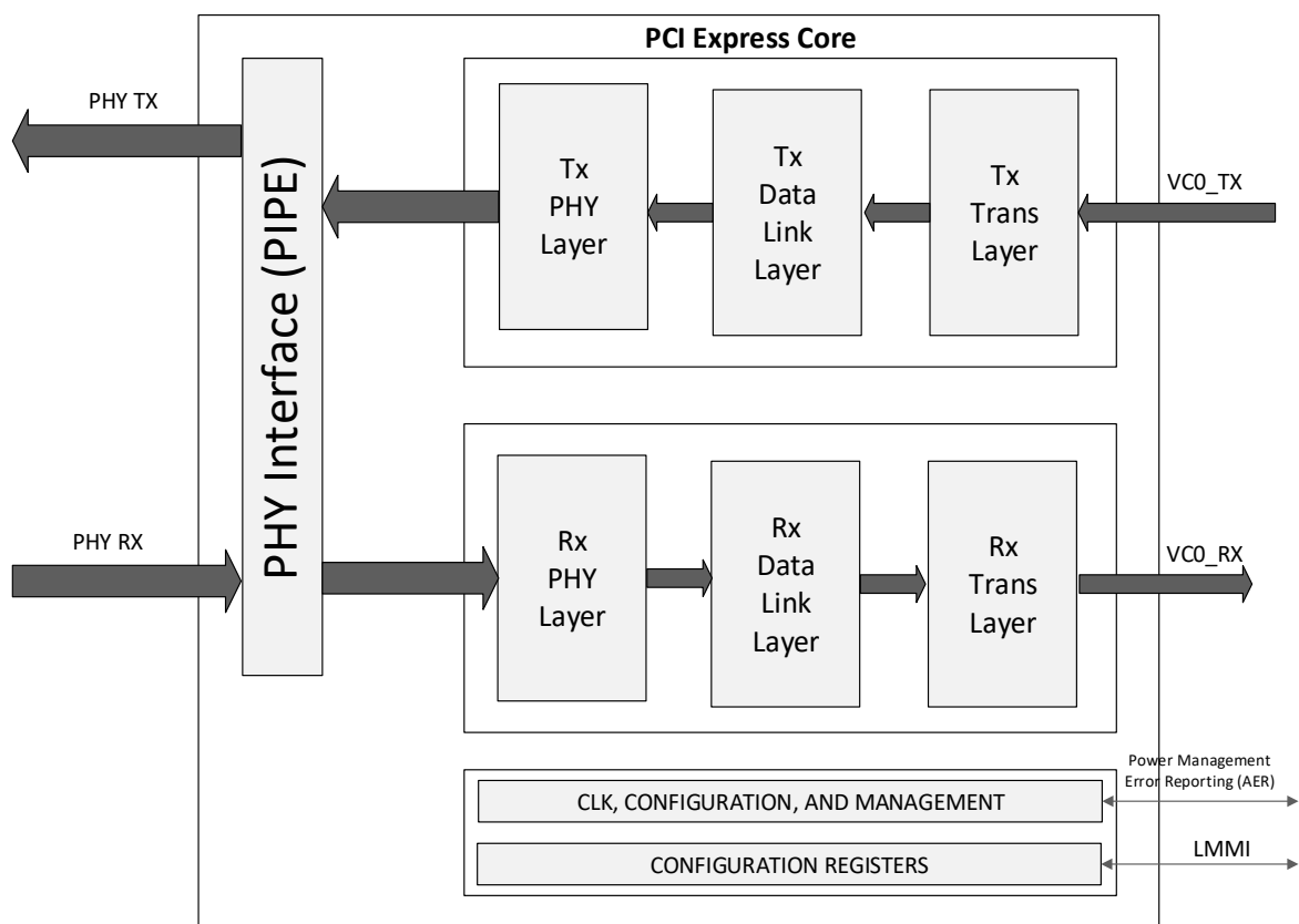
Figure 2.33. PCIe Core
