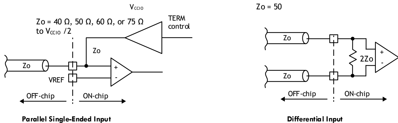
Figure 4.1. On-Chip Termination
