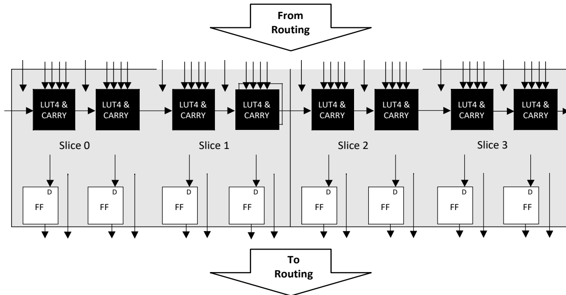
Figure 2.4. PFU Diagram
