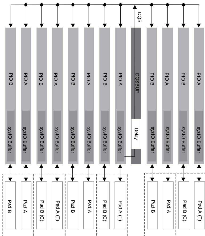
Figure 2.29. DQS Grouping on the Bottom Edge
