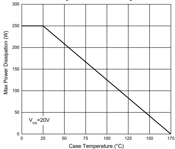
Fig. 13 - Power Derating
