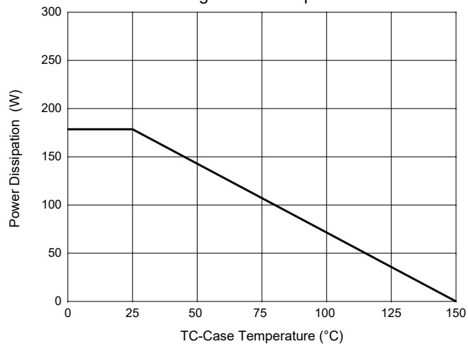
Fig.11-PD-Dissipation
