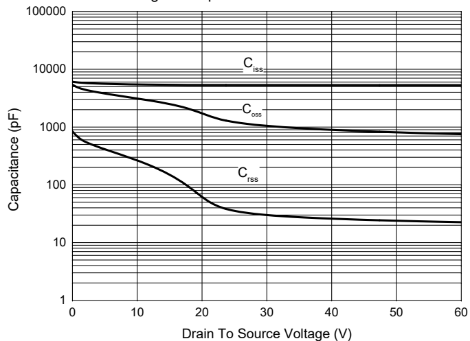
Fig. 5 - Capacitance Characteristics
