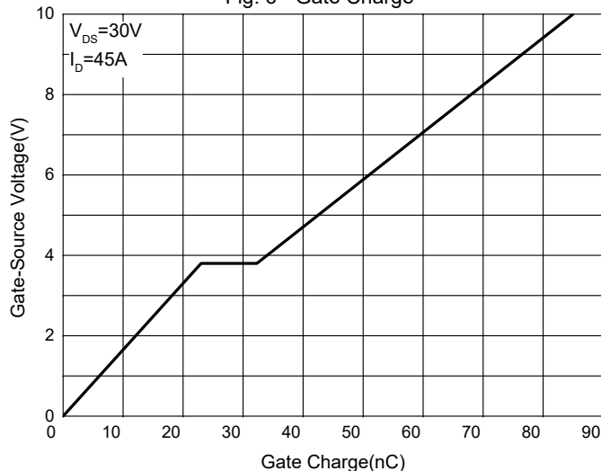
Fig. 6 - Gate Charge
