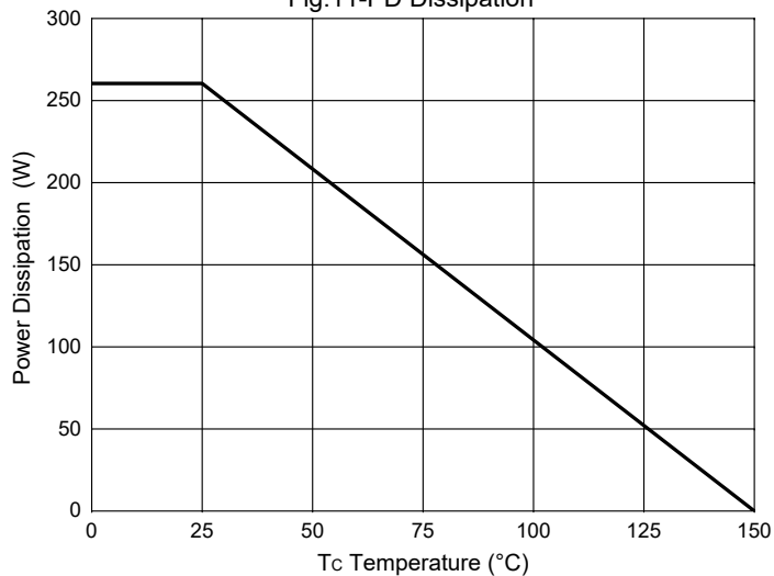
Fig.11-PD Dissipation
