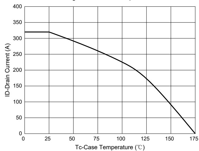
Fig. 10 - Current dissipation
