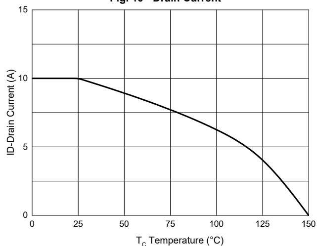
Fig. 10 - Drain Current
