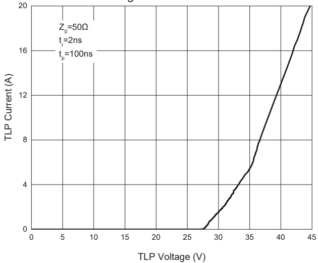
Fig. 5 - TLP Curve
