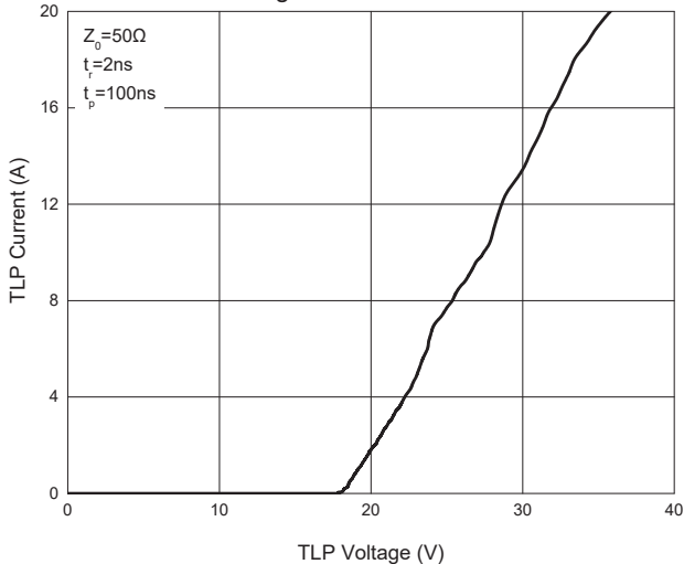
Fig. 5 - TLP Curve
