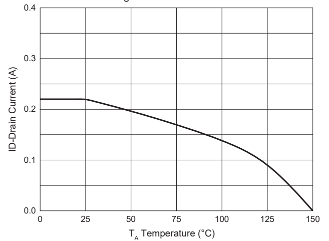
Fig. 10 - Drain Current
