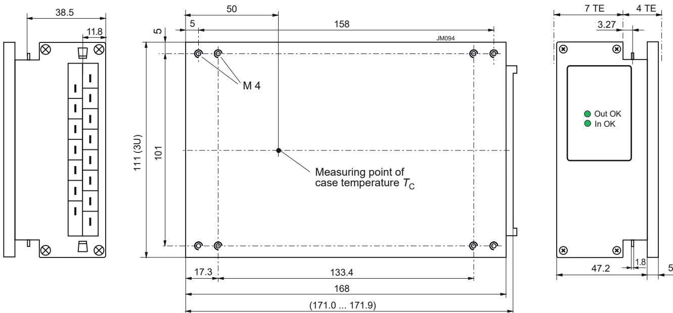
Option B1: Aluminum case S03 with small cooling plate; black finish (EP powder coated). Suitable for mounting with access from the backside. Total weight approx. 1.4 kg.
