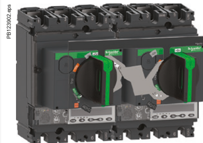
Interlocking of two devices by rotary handles
