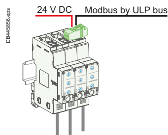
Power supply, with the Communication function, via the Modbus interface
