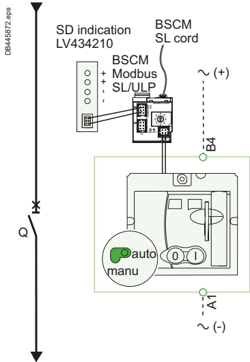
Schematic representation of the communicating motor mechanism (MT).
