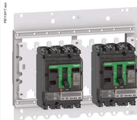
Interlocking on a base plate
