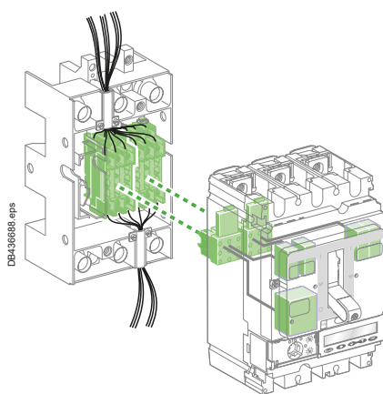
Plug-in/withdrawable ComPacT NSX
