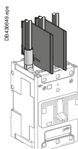
Interphase barriers
