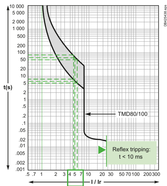
Example 1. Fault I = 500\text{ A}
