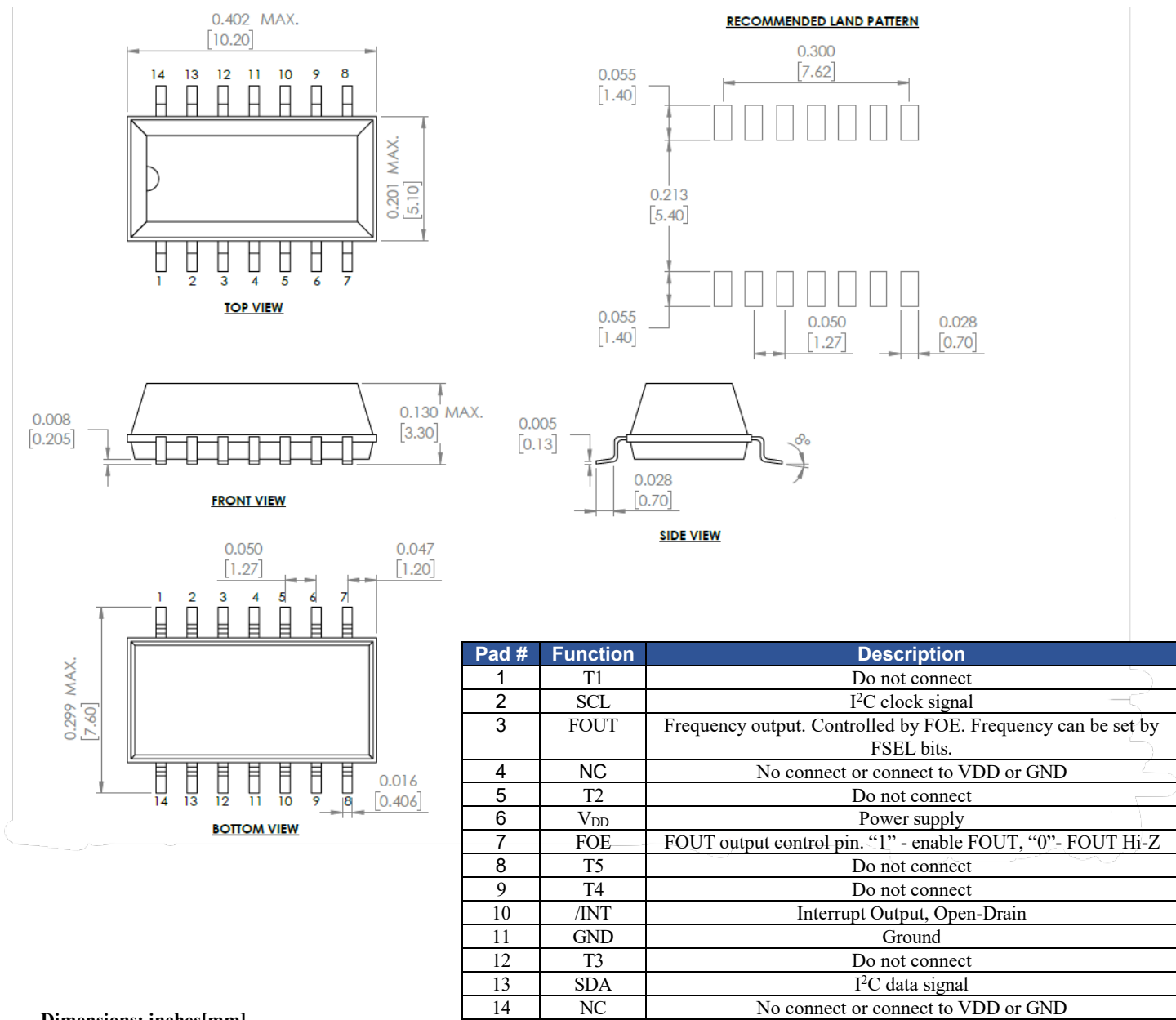
Dimensions: inches[mm]
