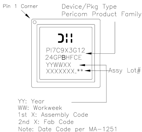
Figure 14-2 Part Marking
