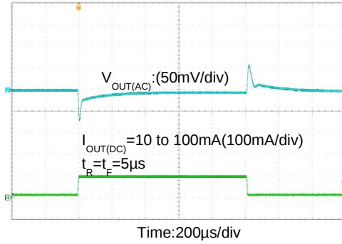
Load Transient Response V_{OUT}=5V
