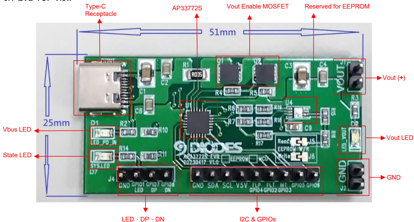
Figure 3. AP33772S Evaluation Board top view and its key portions
