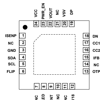
Figure 2. AP33772S Package Outline
