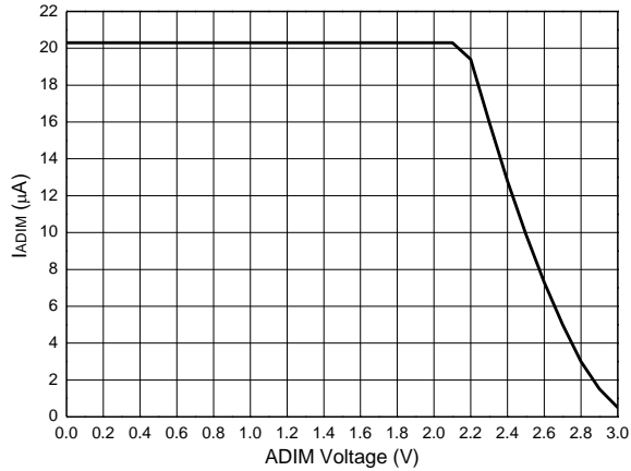
ADIM Sourcing Current vs. ADIM Voltage
