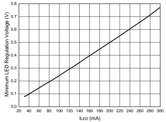
Minimum LED Voltage vs. LED Regulation Current
