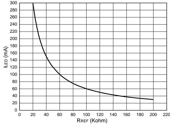
LED Current vs. R_{REF}
