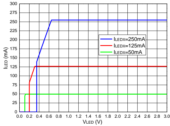
LED Current vs. V_{LED} Voltage
