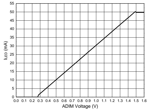
LED Current vs. ADIM Voltage ( R_{REF} = 120\text{k}\Omega , I_{LED} = 50\text{mA} )
