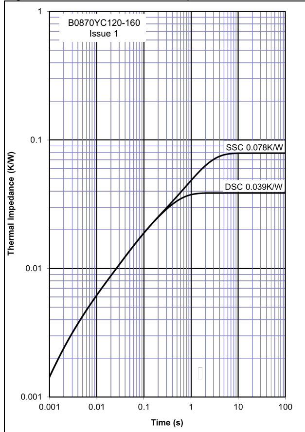
Figure 2 - Transient Thermal Impedance
