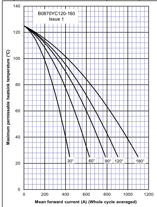
Figure 6 – On-state current vs. Heatsink temperature - Double Side Cooled (Sine wave)
