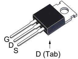
TO-220 (IXFP)
