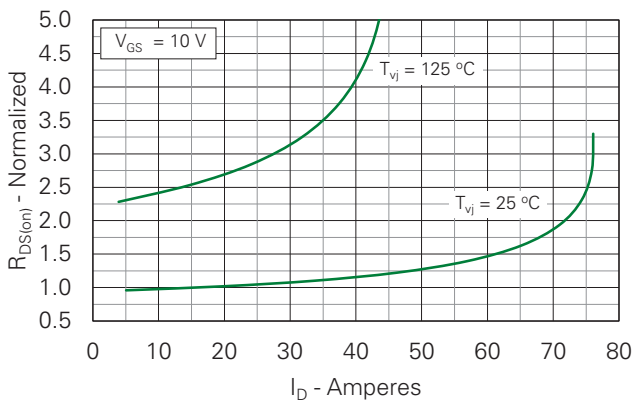
Fig. 5. R_{DS(on)} Normalized to I_D = 17\text{ A} Value vs. Drain Current
