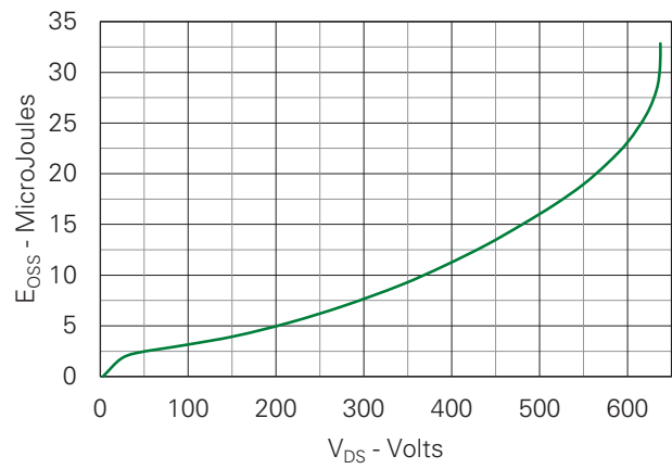
Fig. 13. Output Capacitance Stored Energy
