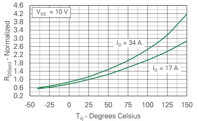
Fig. 4. R_{DS(on)} Normalized to I_D = 17\text{ A} Value vs. Junction Temperature
