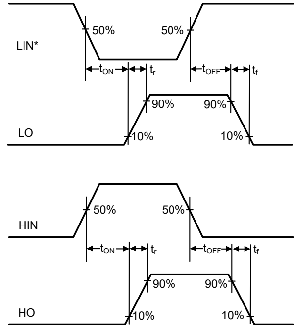
Figure 2. Input-to-Output delay timing diagram
