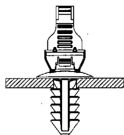
ASSEMBLED VIEW
