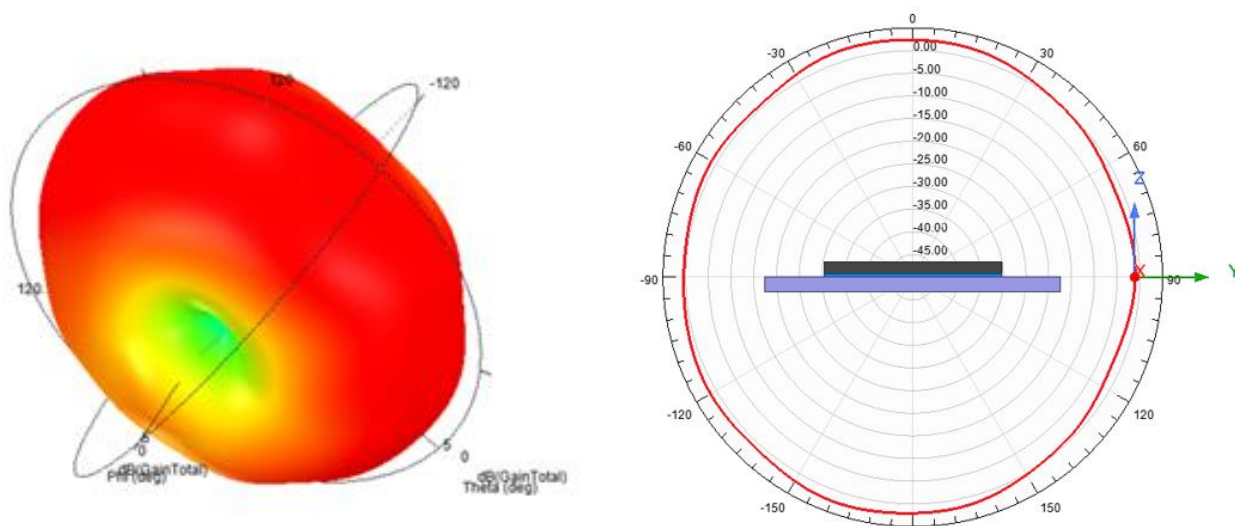
UWB Radiation pattern 2D plot ( \theta , \phi=90^\circ )
