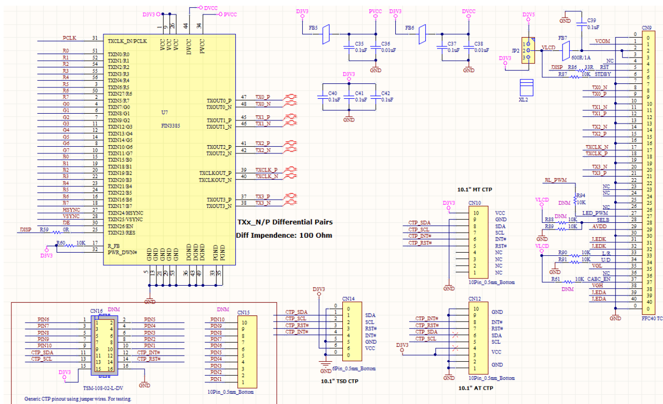
Figure 4-4 - RGB to LVDS converter
