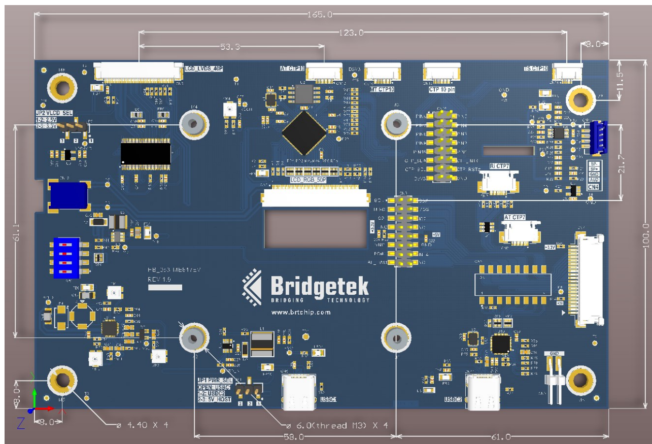
Figure 6-1 - PCB Mechanical Dimensions
