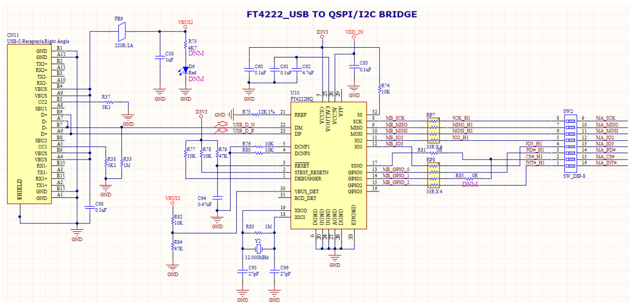
Figure 4-2 - FT4222 USB Bridge Circuit
