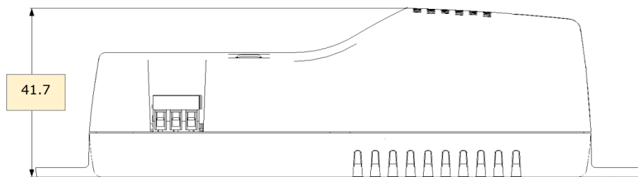
Figure 11 - Modbus Trailing Edge Light Dimmer Dimension – Side View
