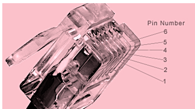
EXP INTERFACE PLUG PINS
