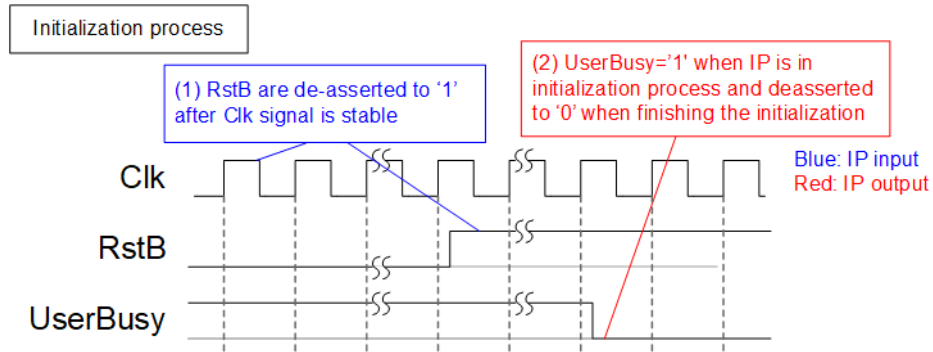
Figure 2: RstB and UserBusy during IP initialization
