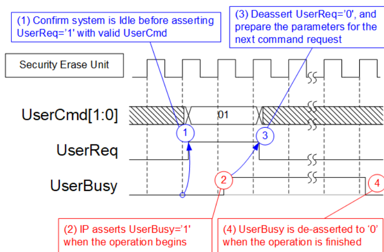
Figure 7: User interface for Security Erase Unit command
