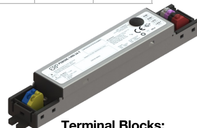
Terminal Blocks: PSBxxExx-T Models L 154.2 x W 26.2 x H 21.85 mm (L 6.07 x W 1.03 x H 0.86 in.)
