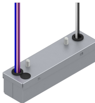
Bottom Leads with Studs: Models with “-S” Suffix L 98.5 x W 26.0 x H 23.7 mm (L 3.88 x W 1.02 x H 0.93 in.)
