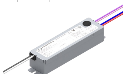
Side Leads: PSBxxW Models L 98.5 x W 26.0 x H 21.85 mm (L 3.88 x W 1.02 x H 0.86 in.)
