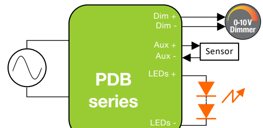
Typical Application Diagram
