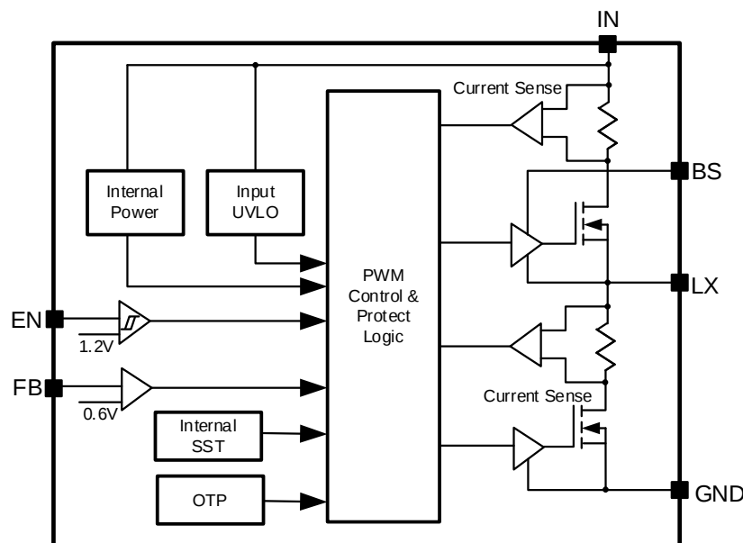
Figure 3. Block Diagram
