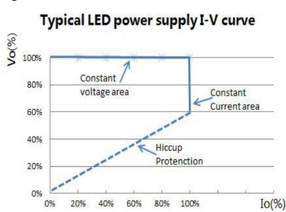
Fig.3 I-V Curve:
