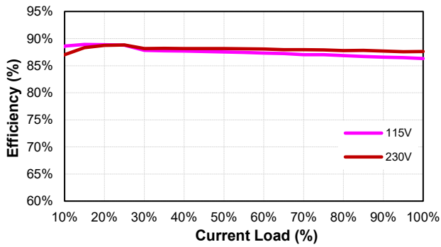
TRH70A240 (Eff Vs Io)
