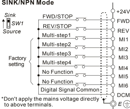
Figure 3 Wiring for SINK(NPN) mode and SOURCE(PNP) mode
