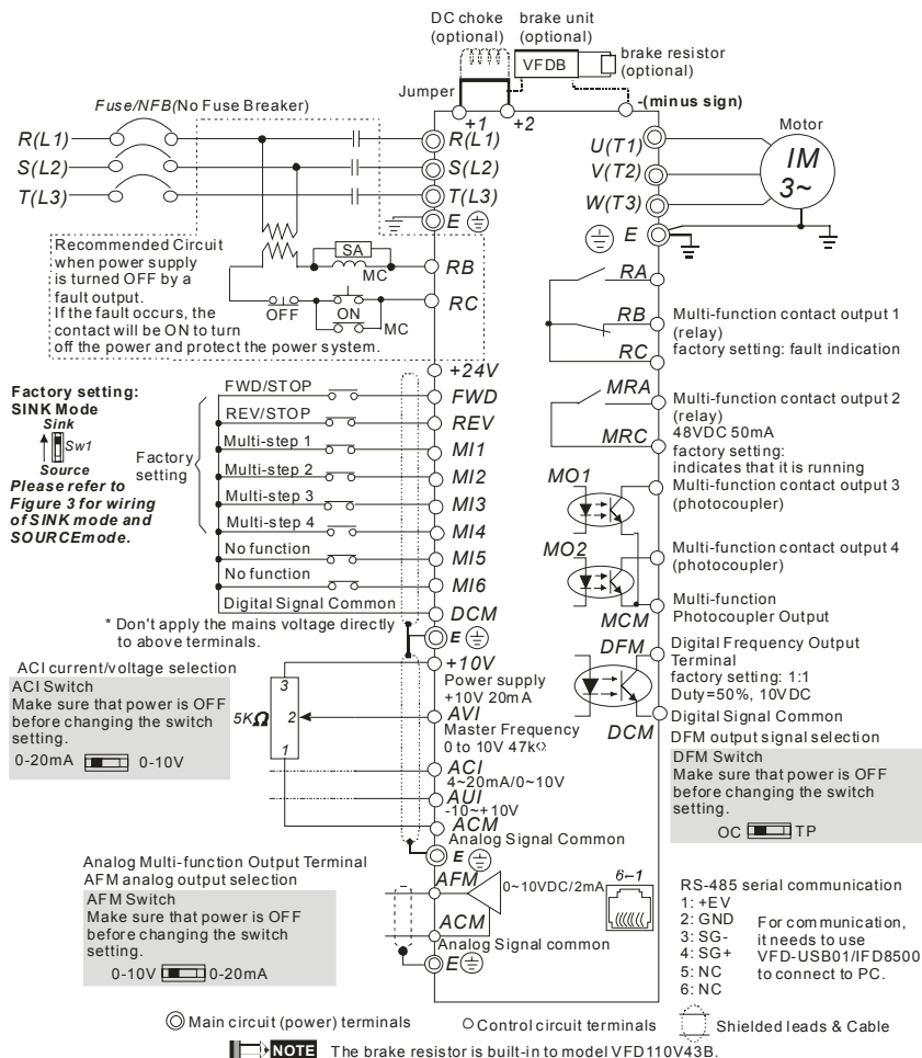
Figure 2 for models of VFD-VE Series (20HP/15kW and above)
