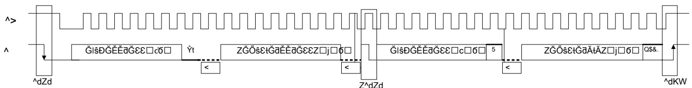
Figure 27. Read Cycle
