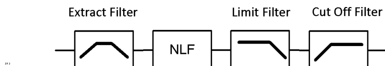
Figure 12. Bass Enhancement
