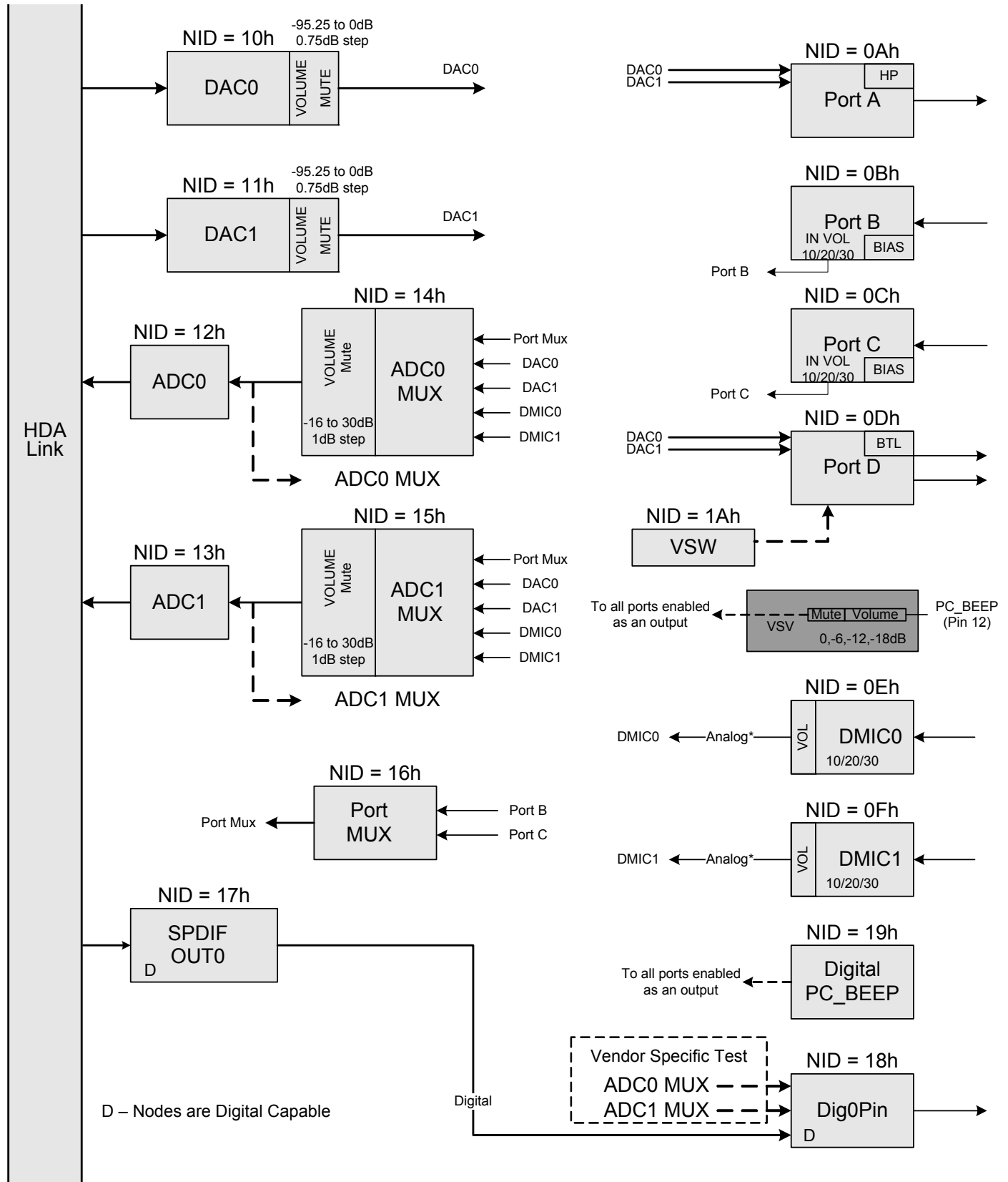
Figure 13. Widget Diagram
