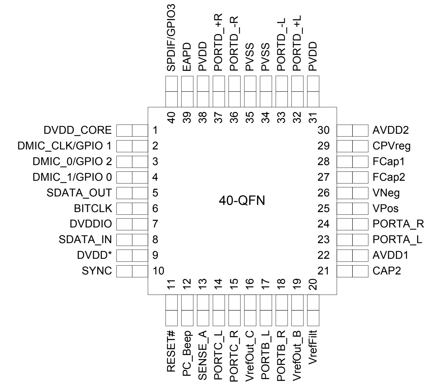
Figure 15. 40-QFN Pin Assignment
