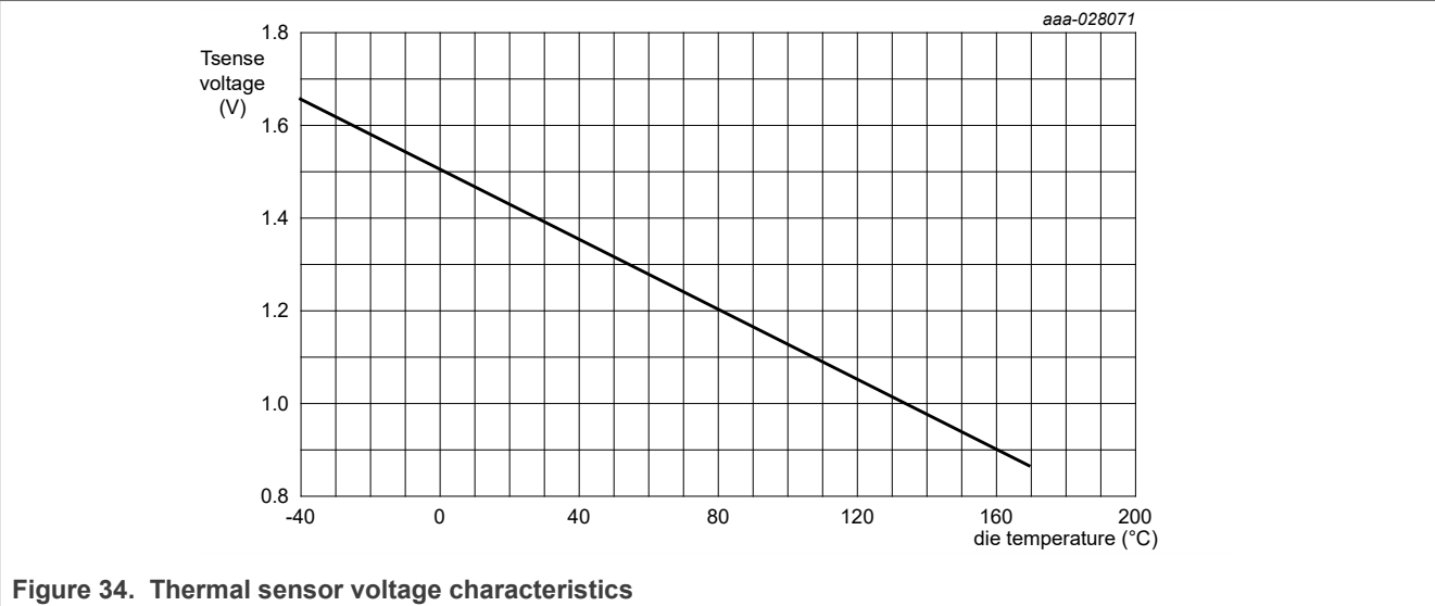
Figure 34. Thermal sensor voltage characteristics
