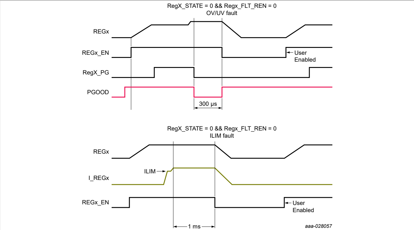
Figure 12. Regulator turned off with RegX_STATE = 0 and FLT_REN = 0
