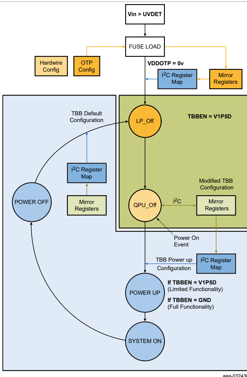
Figure 39. TBB operation diagram
