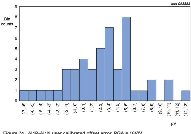
Figure 74. Al1P-Al1N user calibrated offset error, PGA = 16V/V
