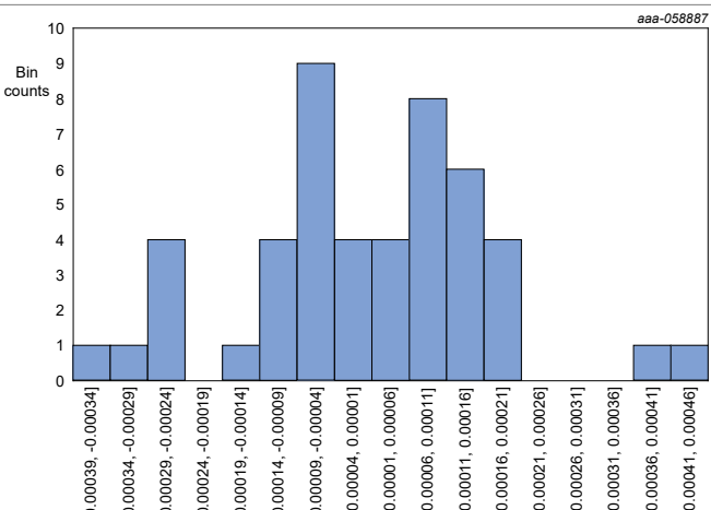
Figure 76. Vsense user calibrated TUE
