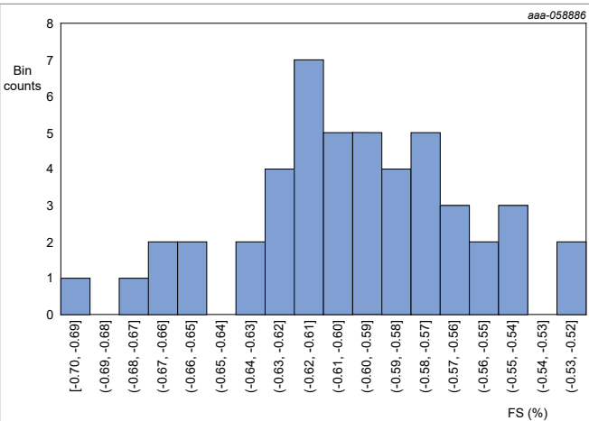
Figure 77. Vsense uncalibrated gain error
