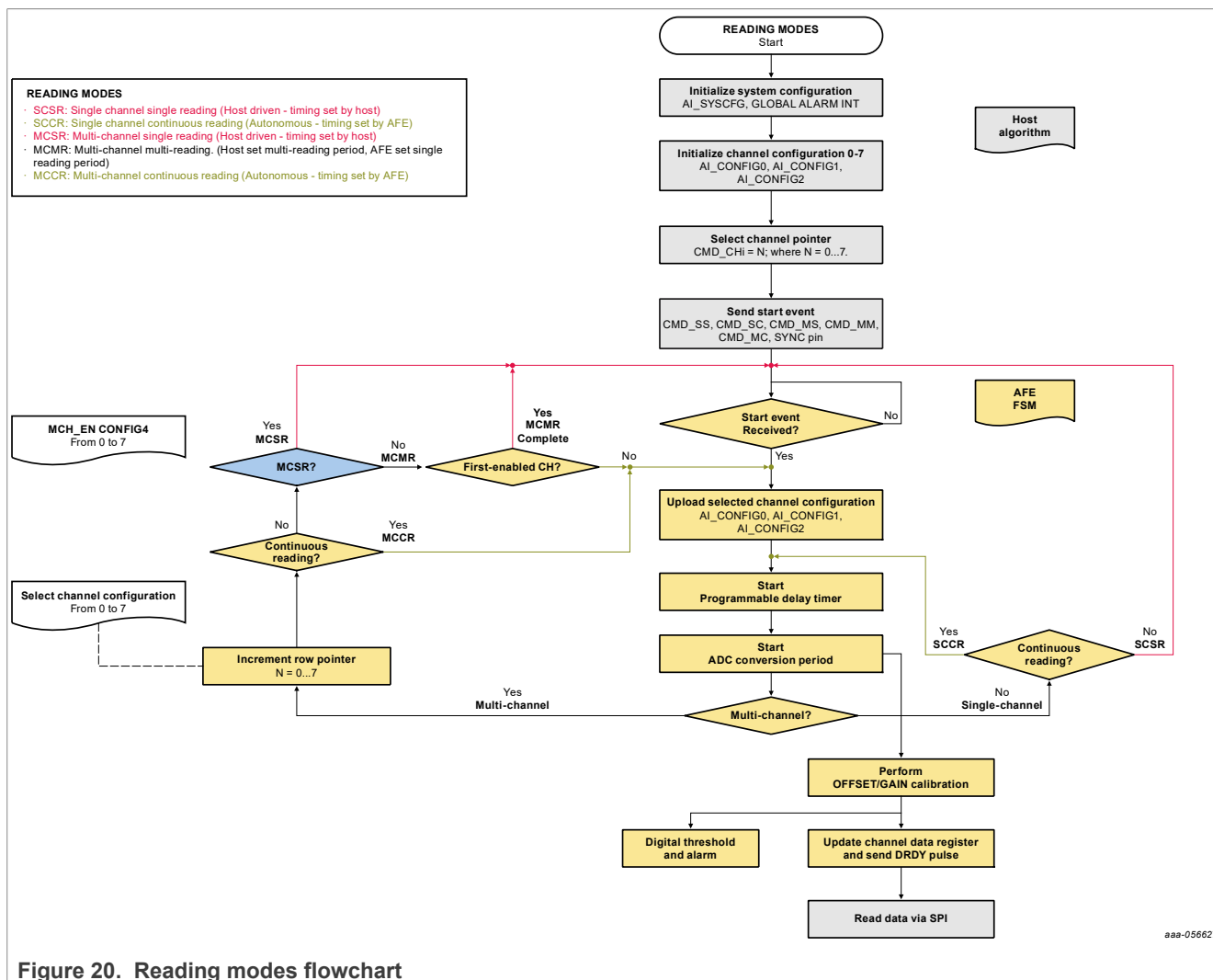
Figure 20. Reading modes flowchart
