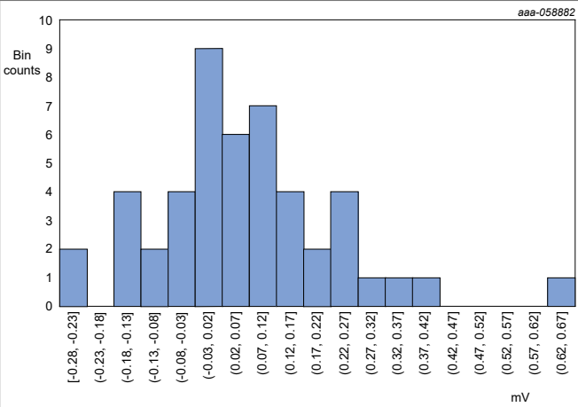
Figure 73. Al1P-Al1N uncalibrated offset error, PGA = 16V/V
