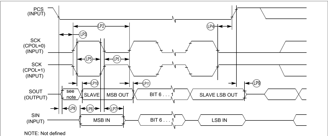
Figure 21. LPSPi peripheral mode timing (CPHA = 1)
