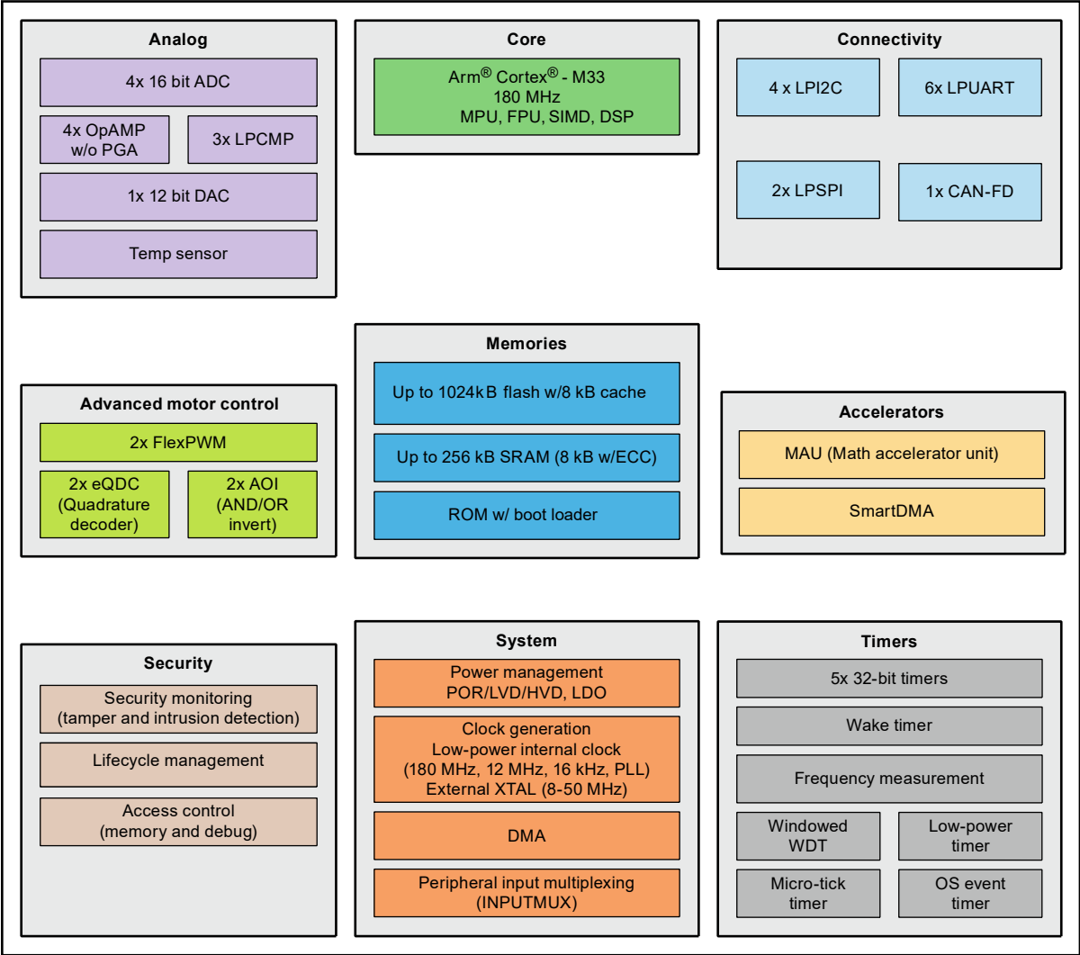
Figure 1. Block Diagram
