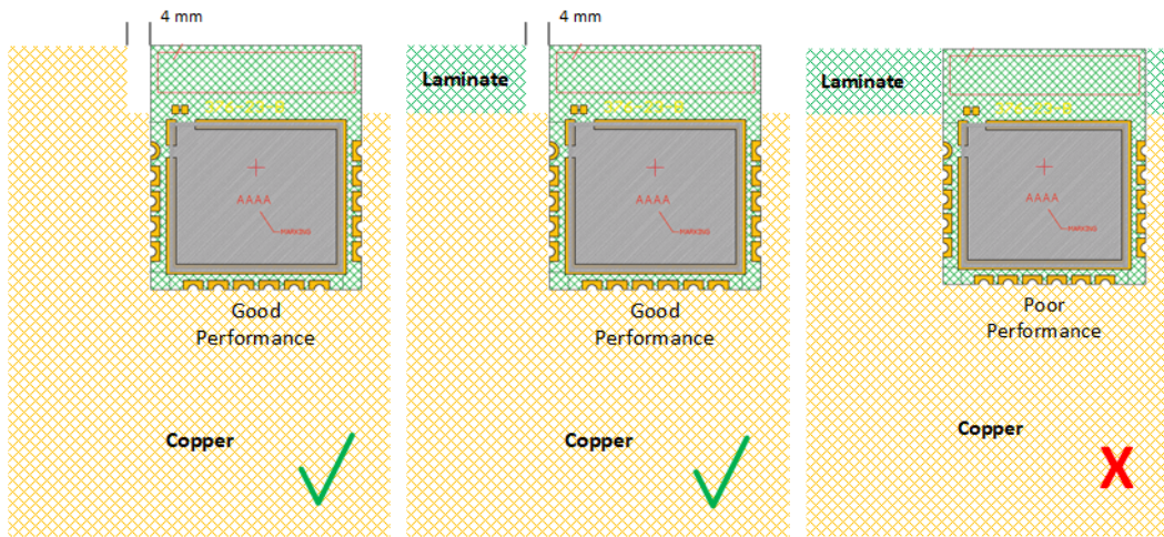
Figure 10. Antenna performance in proximity of copper (left), laminate (middle), and laminate under antenna (right) The actual TINY™ module evaluation board layout that has been used to conduct measurements is shown in Figure 11.
