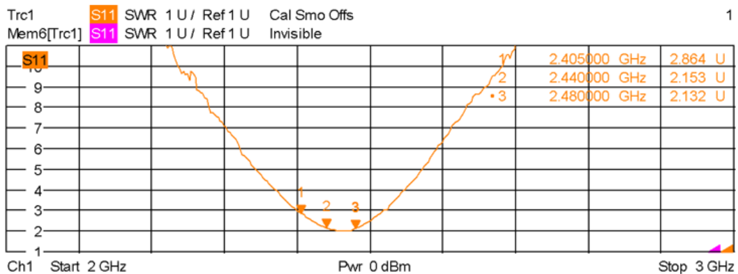
Figure 14. VSWR with module installed in upper-right corner (position #3) of the evaluation board
