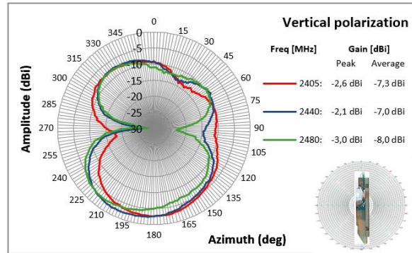
Figure 19. Radiation pattern for XZ-plane, vertical polarization
