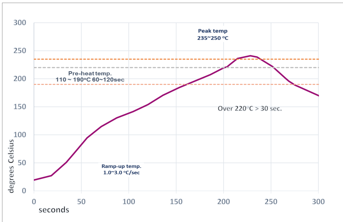
Figure 22. Recommended reflow profile for lead free solder
