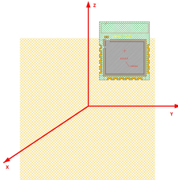
Figure 15. Measurement plane definition
