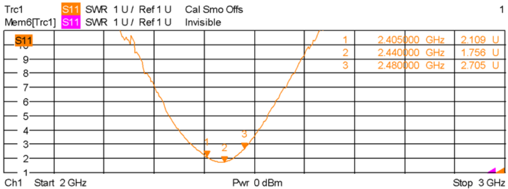
Figure 13. VSWR with module installed in center (position #2) of the evaluation board
