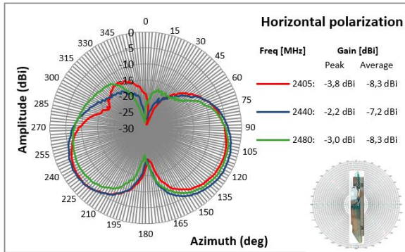
Figure 18. Radiation pattern for XZ-plane, horizontal polarization
