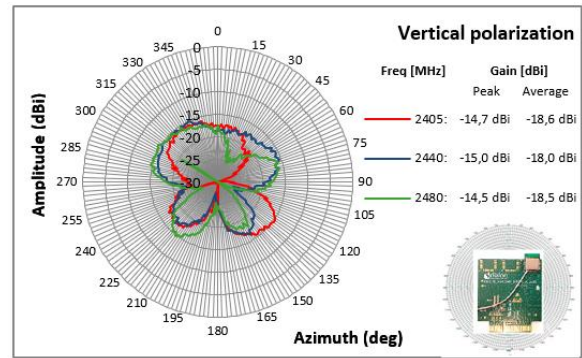
Figure 21. Radiation pattern for YZ-plane, vertical polarization
