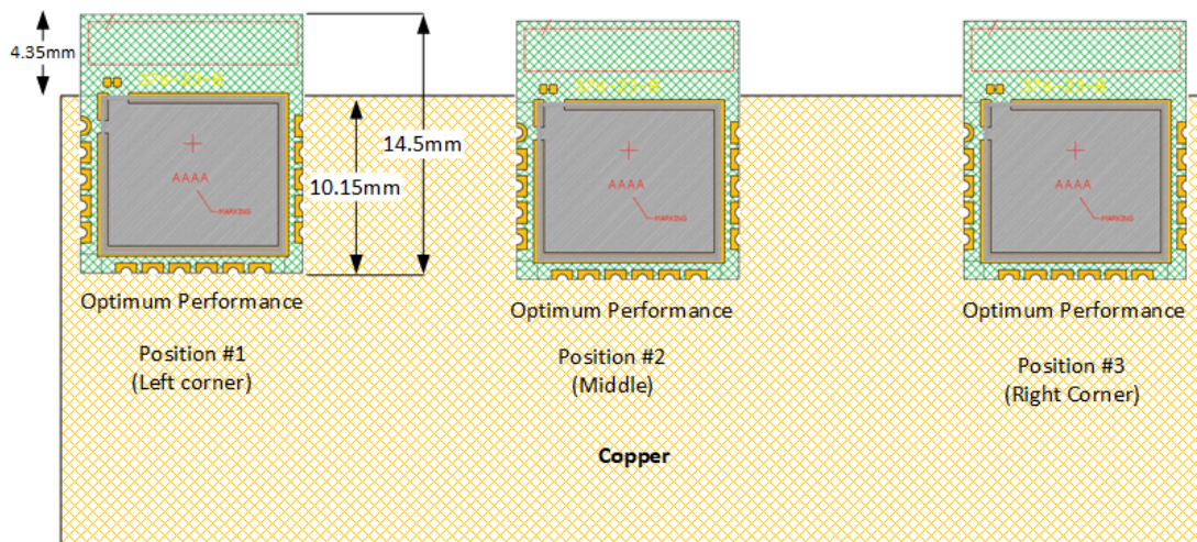
Figure 9. Installation locations for optimum antenna performance
