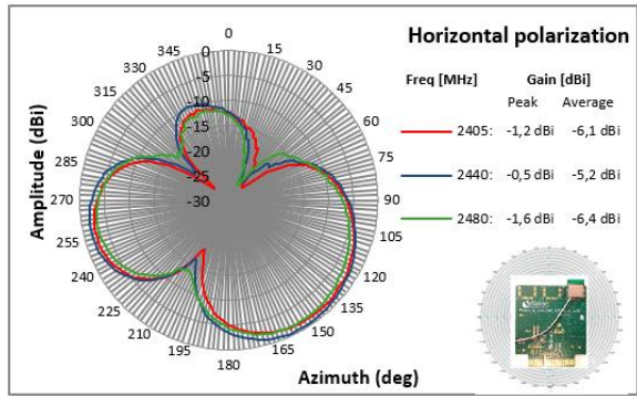
Figure 20. Radiation pattern for YZ-plane, horizontal polarization
