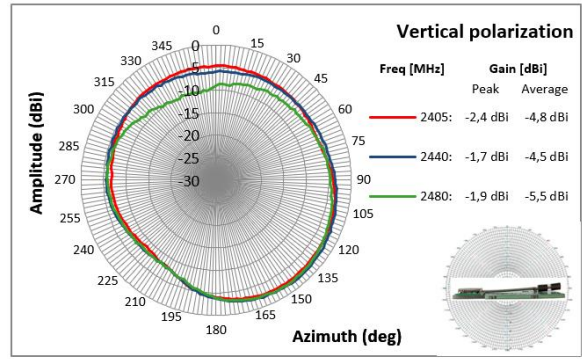
Figure 17. Radiation pattern for XY-plane, vertical polarization
