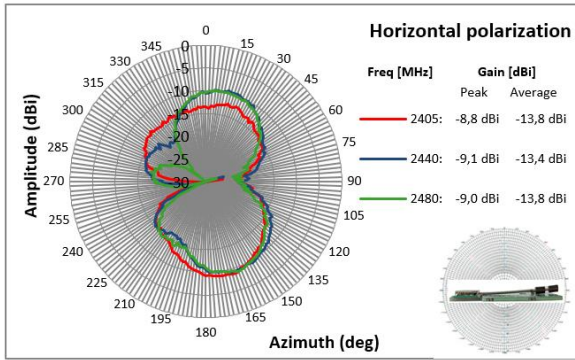
Figure 16. Radiation pattern for XY-plane, horizontal polarization
