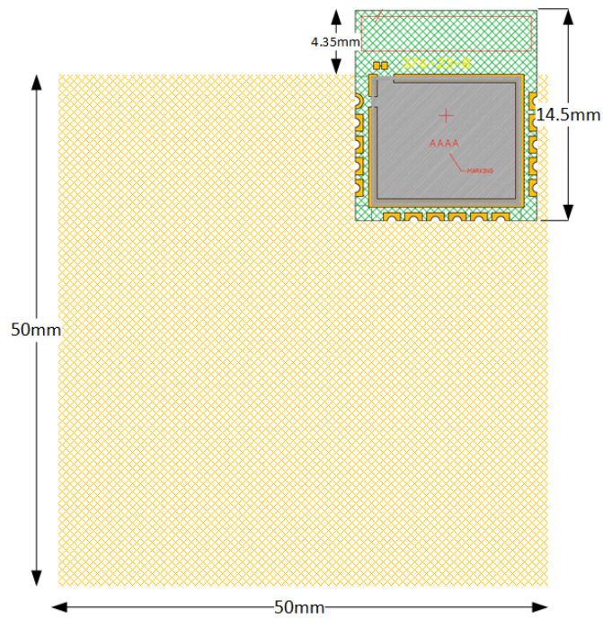
Figure 11. DA14531 TINY™ module evaluation board
