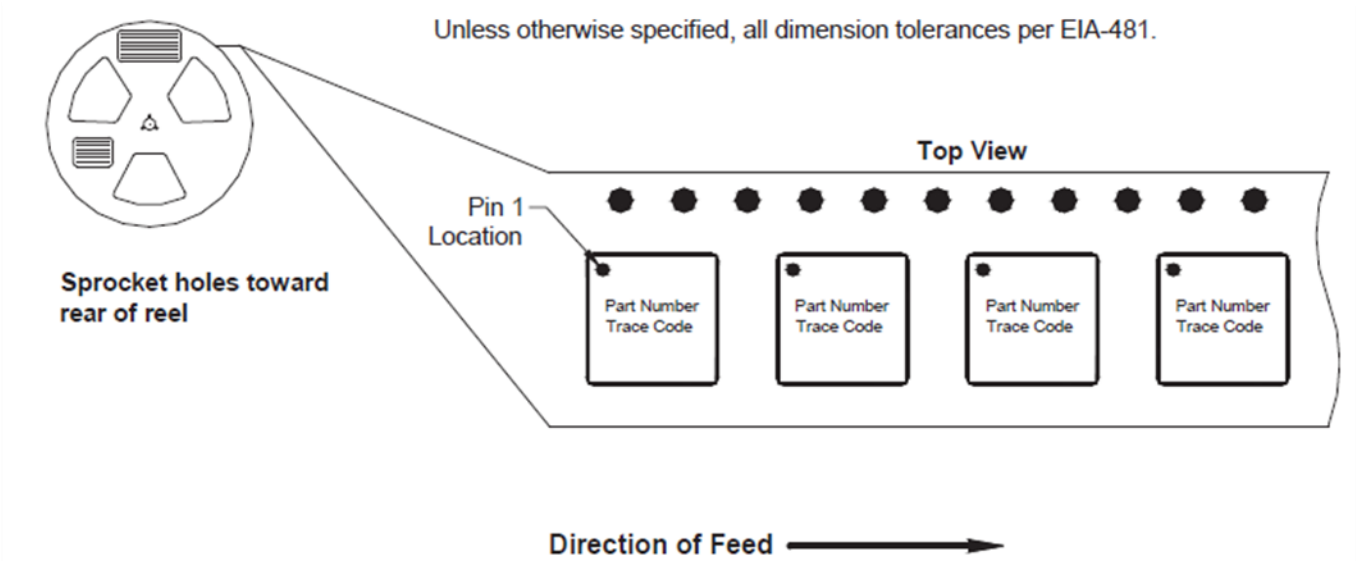
3.0mm x 3.0mm Carrier Tape Drawing with Part Orientation
