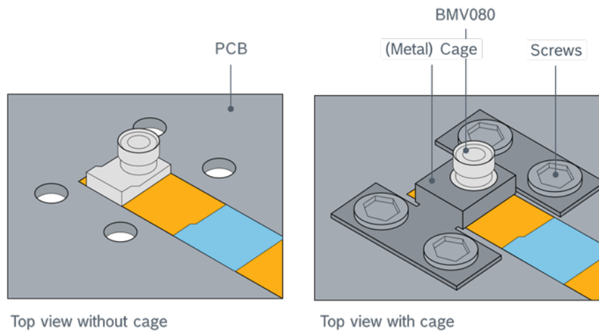
Figure 18: Concept 2 – PCB mounting
