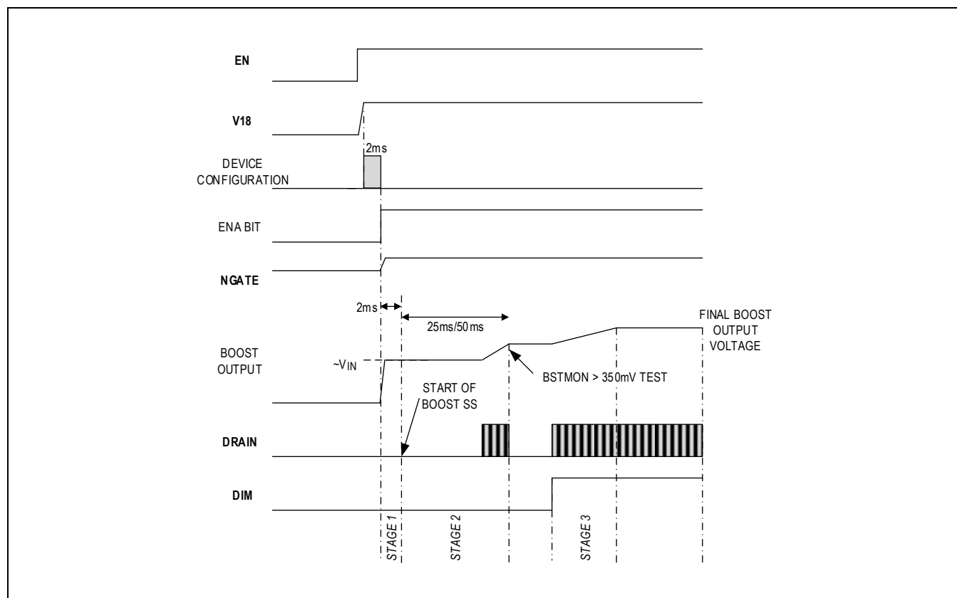
Figure 1. Start-up Sequence
