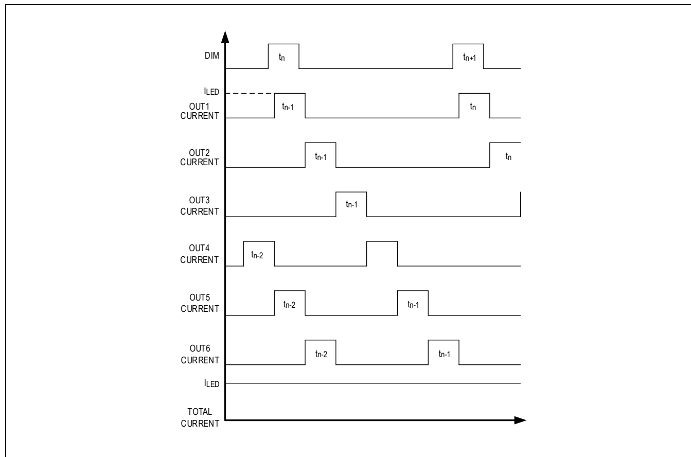
Figure 2. Phase-Shifted Outputs
